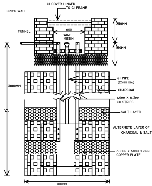
COPPER PLATE EARTHING
