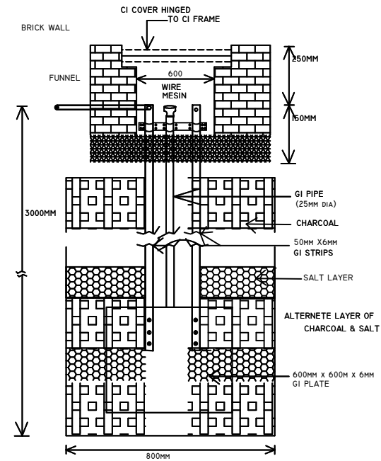
GI PLATE EARTHING
